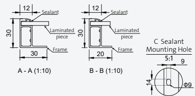
Cross Section A-A & B-B
