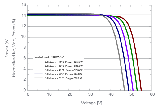
I-V Characteristics At Different Temperatures
