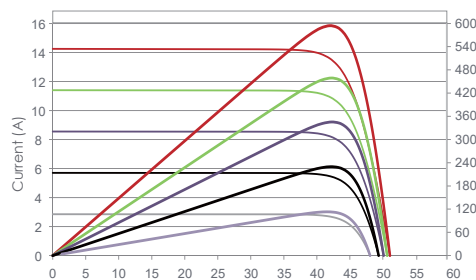
Current-Voltage & Power-Voltage Curves ( 600W)
